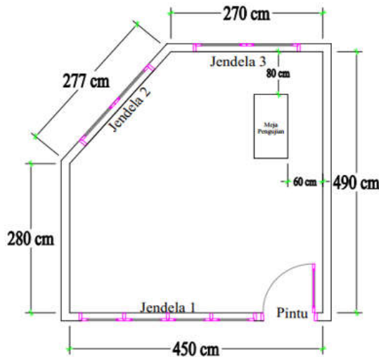
Gambar 2. Denah ruang penelitian.
