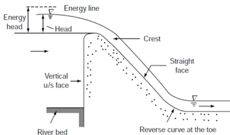
Gambar 5. Ogee Spillway
