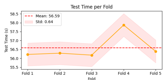
Gambar 5. Hasil Test Time 5 Fold
