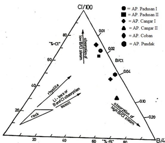
Gambar 3. Diagram ternary geoindikator Cl/100–Li-B/4
