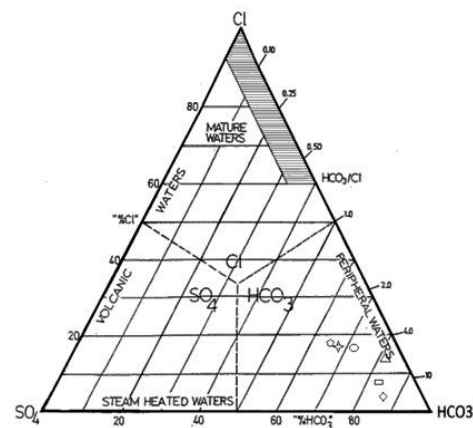
Gambar 2. Diagram ternary geoindikator Cl-SO 4 -HCO 3
