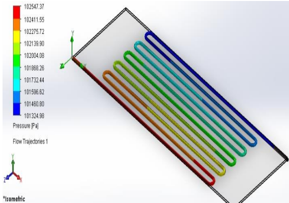
Gambar. 7. Hasil Simulasi pressure drope Kolektor surya W 40 mm rangkaian vertical sambungan U-bend.
