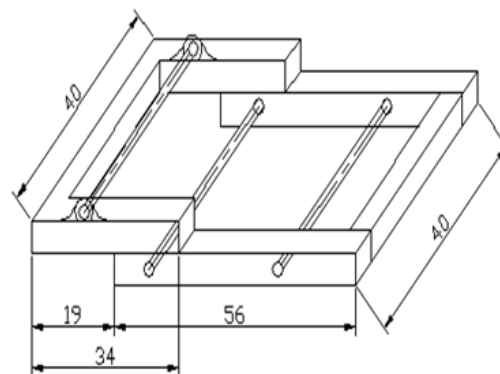
Fig 1. The Top part of Frame
