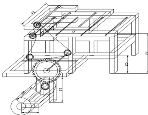
Fig 4. The Pressing Machine of banana sale
