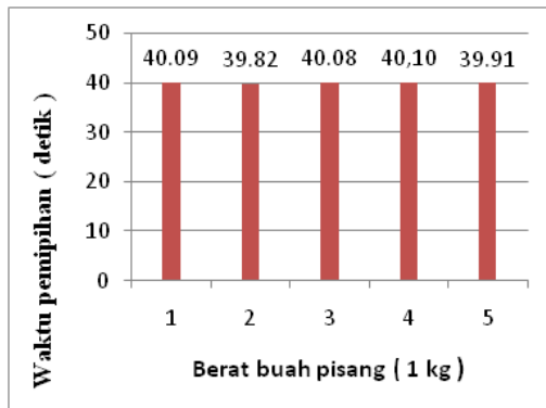
Fig. 8. Time of pressing (second)
