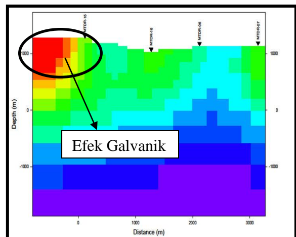
Gambar 8. Efek galvanic model 2D line 2 .
