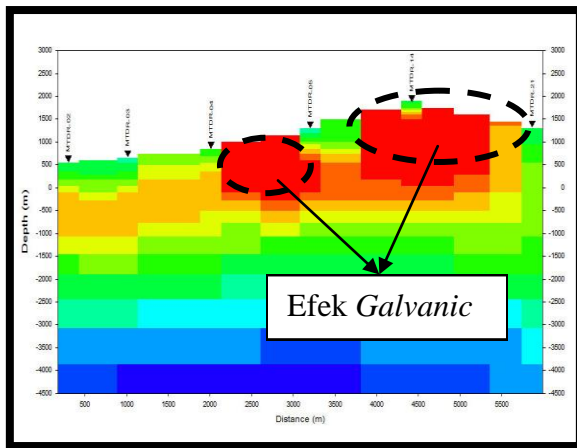
Gambar 6. Efek galvanic model 2D line 1 .
