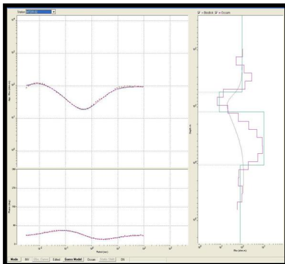
Gambar 5. Kurva Bostick 1D.
